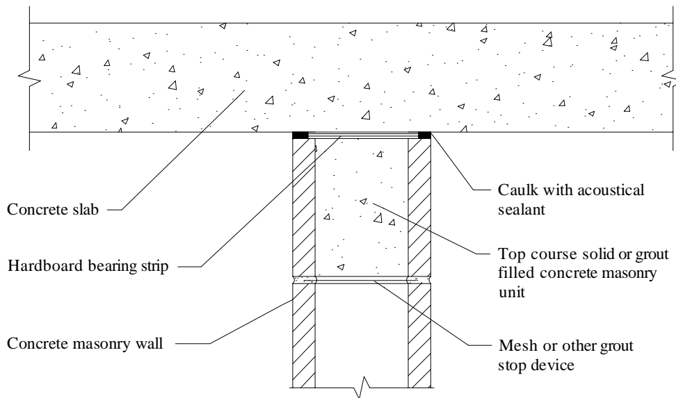
(b) Bearing Wall
