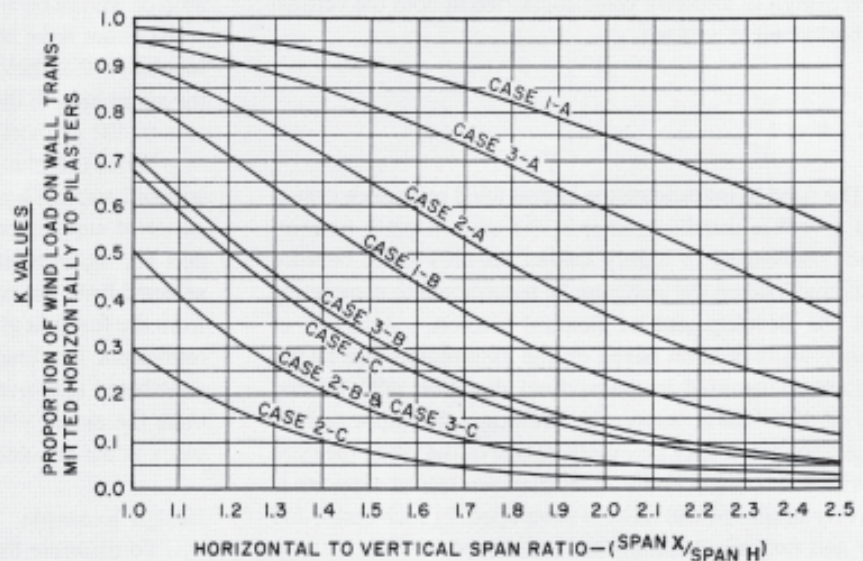
Figure 1—Approximate Horizontal and Vertical Wind Load Distribution
