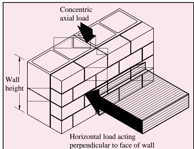
Figure 1—Concentric Axial and Lateral Loading
